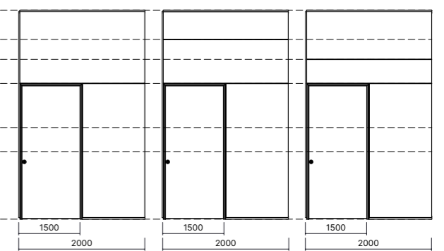
RH/LH SINGLE SLIDING DOORS PORTE SCORREVOLI SINGOLE DX-SX
